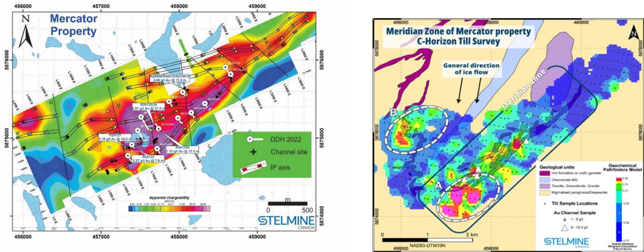
Figure 8. Strong till anomalies detected by the sum of pathfinder elements (2Cu+2As+Au) using the Inverse Distance weighted Interpolation (IDW) method. Anomaly A identifies the Meridian Zone and detects a down-ice dispersion trail from the core of mineralization. Anomaly B straddles iron formations exposures in a less explored area.
