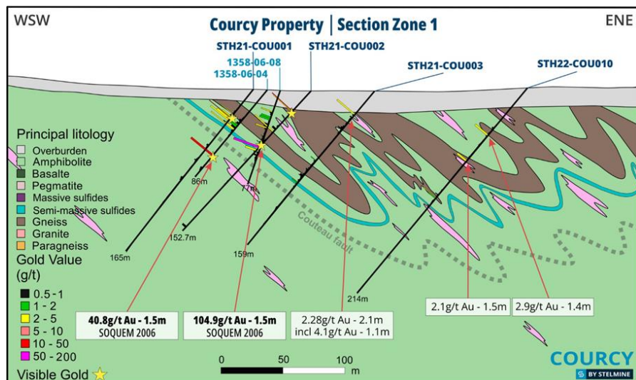
Fig. 4: Section WSW-ENE incluant 6 forages, avec la distribution de la minéralisation aurifère, incluant la structure principale de la Zone 1 de la propriété Courcy. / WSW-ENE section including 6 drill holes, with distribution of gold mineralization, including the main gold-bearing structure on Zone 1 on the Courcy property.
