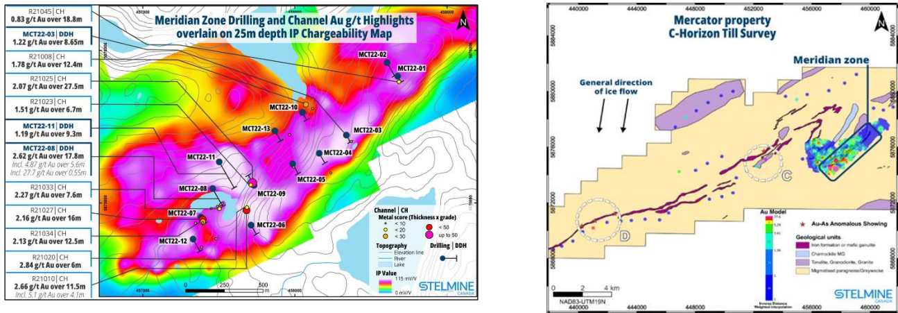
Figure 9. Gold till anomalies from samples collected west of the Meridian Zone in areas of granulitic iron formation exposures. Anomalies C and D located west of the Meridian zone are associated with iron formation exposures around which grab rock and channel sampling reveal anomalous As et Au concentrations.
