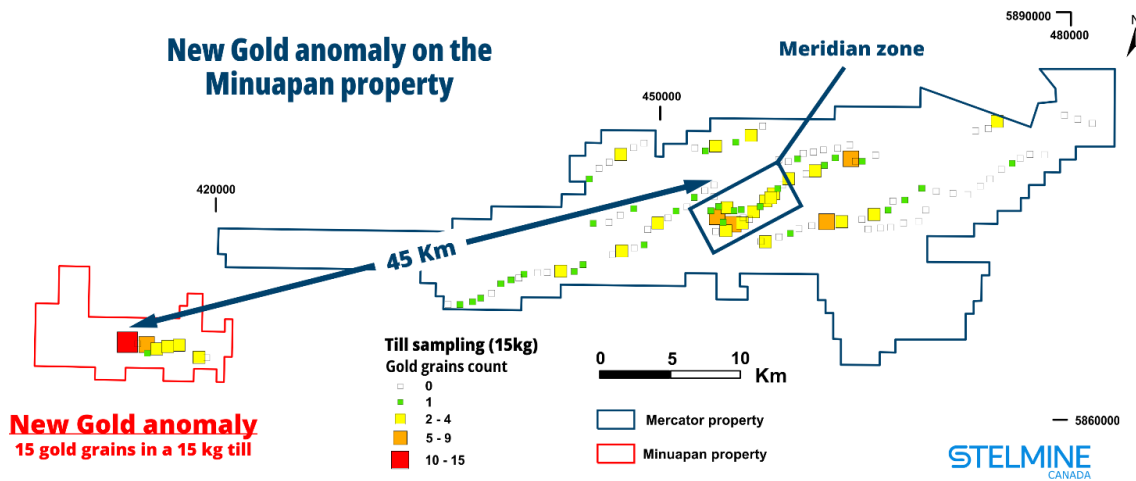
Fig. 1 Claim map of the Mercator and Minuapan properties. Gold grain count from the heavy mineral concentrate (HMC) extracted form 15 kg till material is reported on the map.
