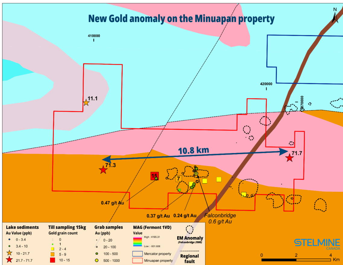
Fig. 2. Claim map of the Minuapan property on a geological background showing the Au geochemical and geophysical anomalies.
